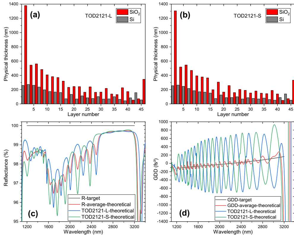
Fig. 2. (a) Layer structure of TOD2121-L. (b) Layer structure of TOD2121-S. (c) Reflectance target, average reflectance upon one bounce and individual reflectance curves of TOD2121-L and TOD2121-S. (d) GDD target, average GDD per bounce as well as individual GDD of TOD2121-L and TOD2121-S.
