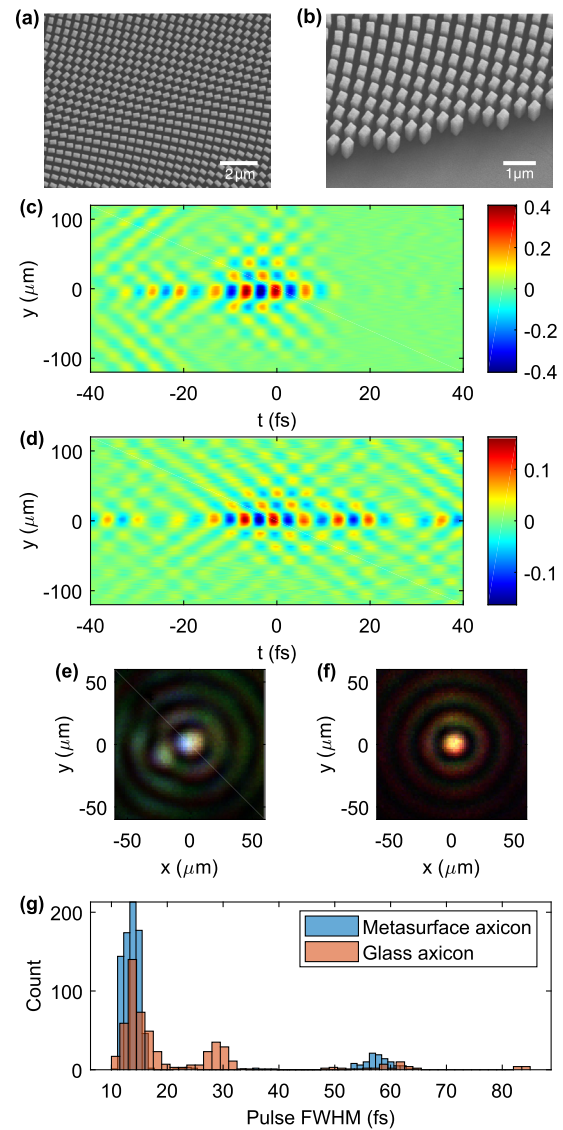
Fig. 3. Characterization of truncated Bessel beams produced by a metasurface axicon and a glass axicon. (a), (b) SEM images of a fabricated meta-axicon comprising amorphous silicon nanofins. (c) Spatiotemporal electric field distribution along the y axis of meta-axicon generated Bessel beam. The numerical aperture of this meta-axicon is about 0.06. Electric field images of the resulting beam were taken with 4\times , 0.1 NA objective. (d) Spatiotemporal electric field distribution produced by a glass axicon of approximately the same numerical aperture. (e) False color image of the Bessel beam produced by the metasurface axicon, where red, green, and blue correspond to frequencies of 135 THz, 164 THz, and 192 THz, respectively. (f) False color image of the Bessel beam produced by the glass axicon. (g) Histogram of pulse durations (full width at half-maximum of intensity) produced by the two axicons.
