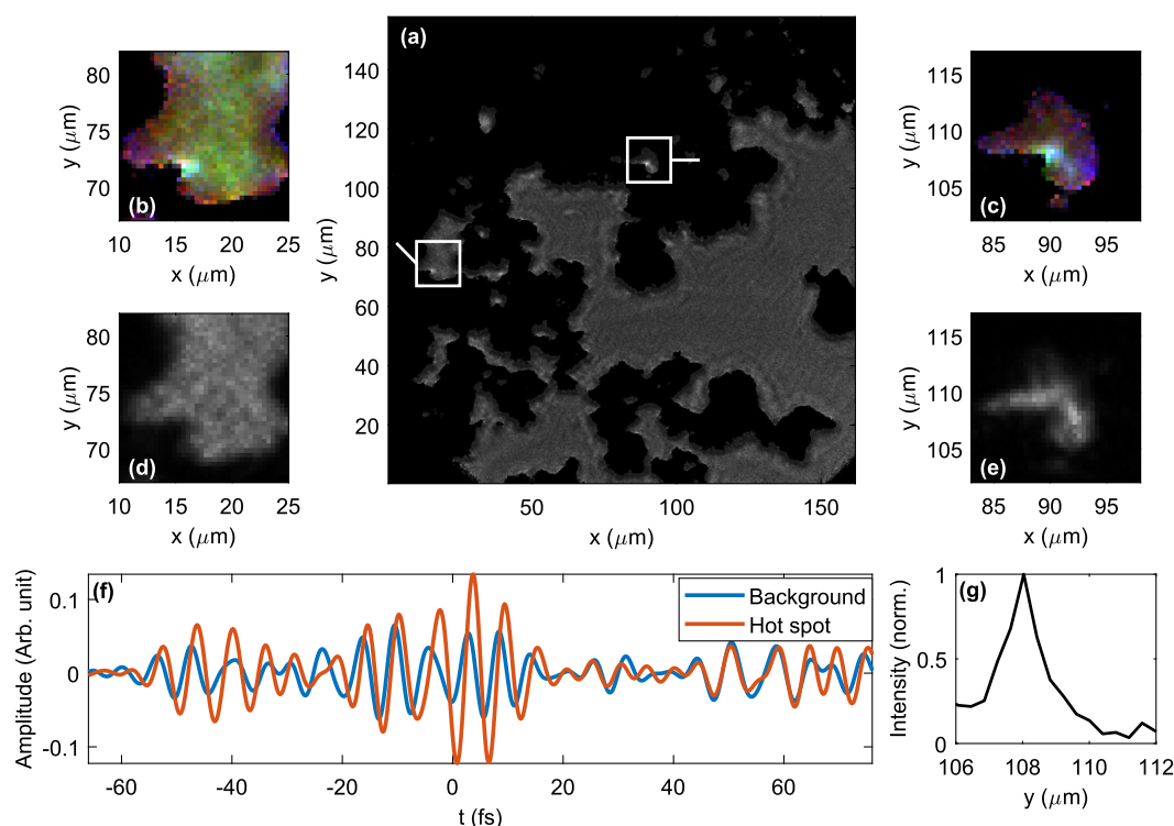
Fig. 4. Sub-wavelength-resolution, time-resolved imaging of the enhanced electric field in the vicinity of aggregated silver-coated fused silica particles. Images were taken with 20 \times , 0.4 NA objective. (a) A wide-field image showing the peak intensity of each recorded waveform. The brightness of each pixel corresponds to the maximum local intensity of the infrared pulse recorded during the temporal window of the measurement. Note that the apparent sharp outline of black areas is due to gating that sets the field of regions with insufficient sampling signal to zero. (b), (c) Zoomed-in views of the enhanced field strength near sharp corners, shown in false color, where red, green, and blue correspond to 145 THz, 165 THz, and 180 THz, respectively. This makes use of the complete spectral information recorded at each sub-wavelength pixel as an additional enhancement of contrast. (d), (e) Corresponding optical transmission images. These images were obtained by the same imaging optics with only the sampling laser as an illumination source. (f) Electric waveforms at two specific pixels in (c) from the location of the brightest pixel and the relatively unperturbed background. This plot shows the temporal profile of the enhanced field. (g) Lineout of the hot spot in (c), with a FWHM of 1.2 \mu\text{m} .
